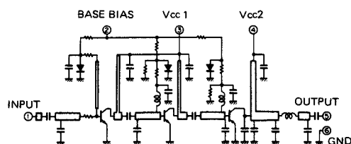
Fig. 5 Power module M57716 Equivalent circuit
