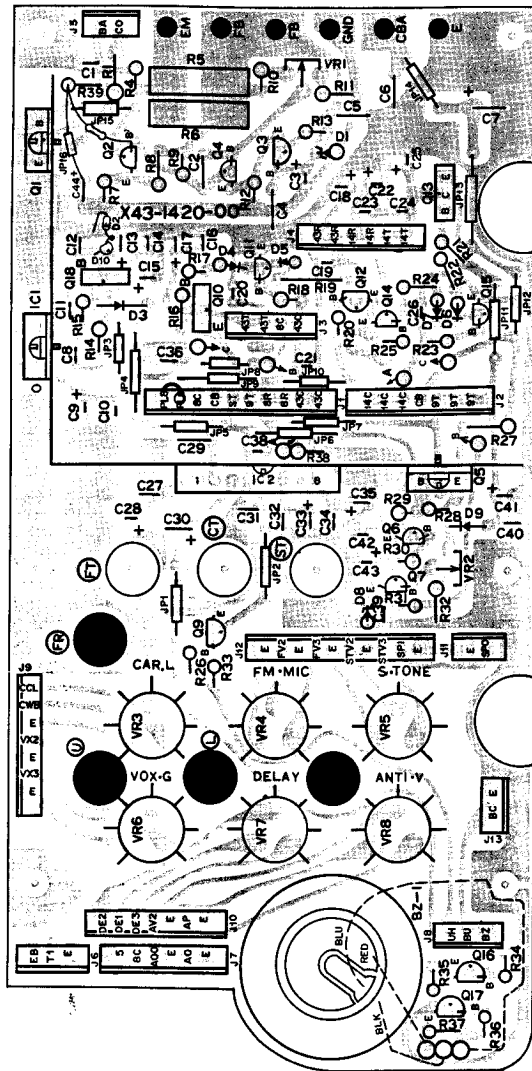
▼ AVR UNIT (X43-1420-00) Components side view
