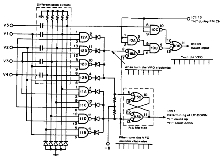
Fig. 14 Encoder waveform shaping
