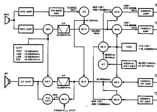
Fig. 1 Block diagram
