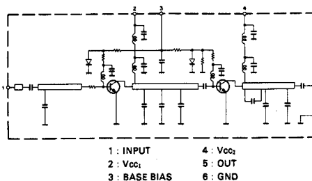
Fig. 4 Power module M57713 Equivalent circuit
