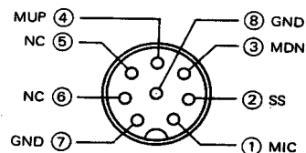
Fig. 17 MIC terminals (view from front panel side)
